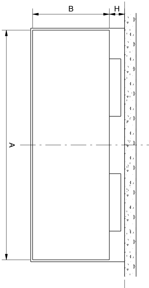
TOP VIEW:
