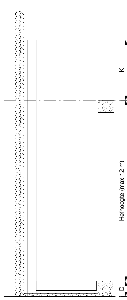
SECTION:
